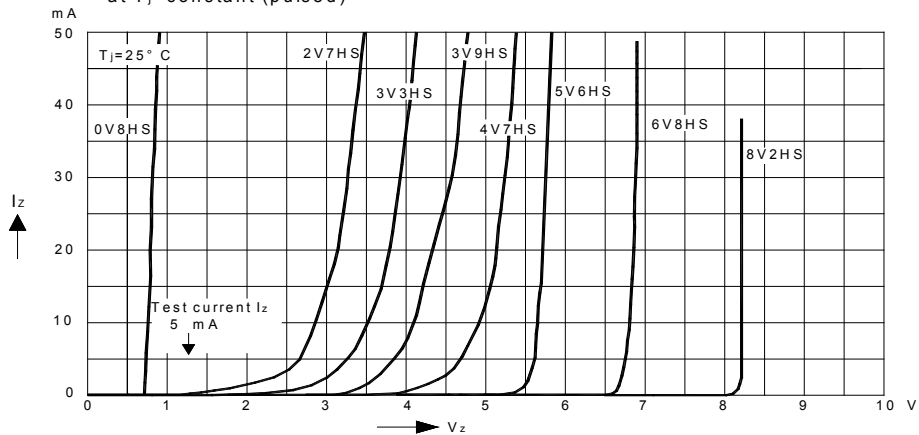
Breakdown Characteristics at T_j = \text{constant} (pulsed)
