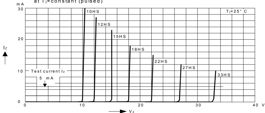
Breakdown Characteristics at T_j = \text{constant} (pulsed)
